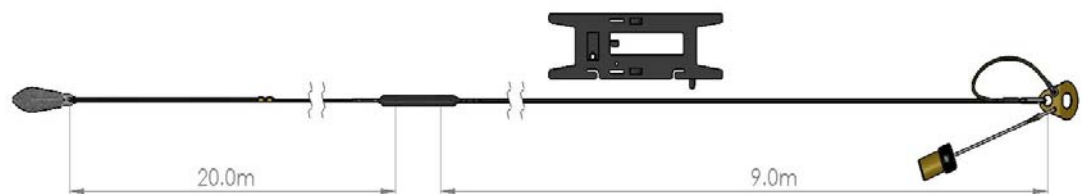
Antenna dimensions
