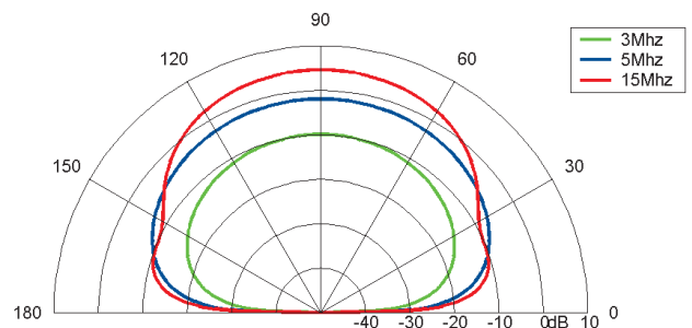
Elevation at 90°
